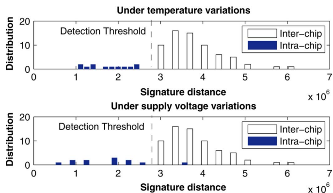
Fig. 14. Distribution of the intra- and interchip signature L_1 distances.
