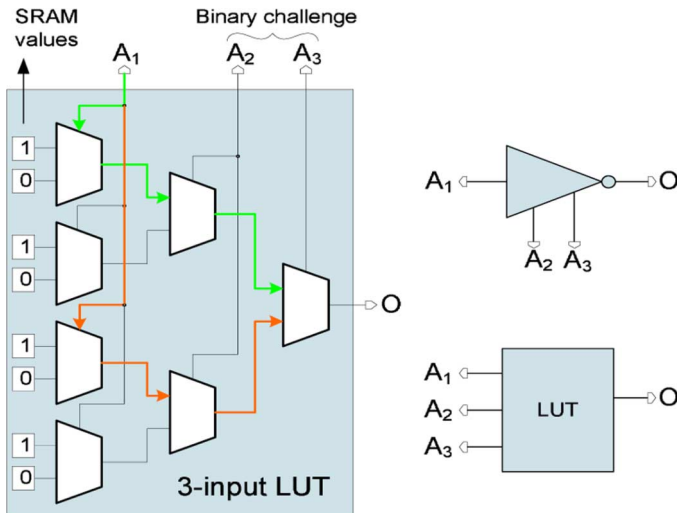
Fig. 5. Internal structure of LUTs. The signal propagation path inside the LUTs change as the inputs change.
