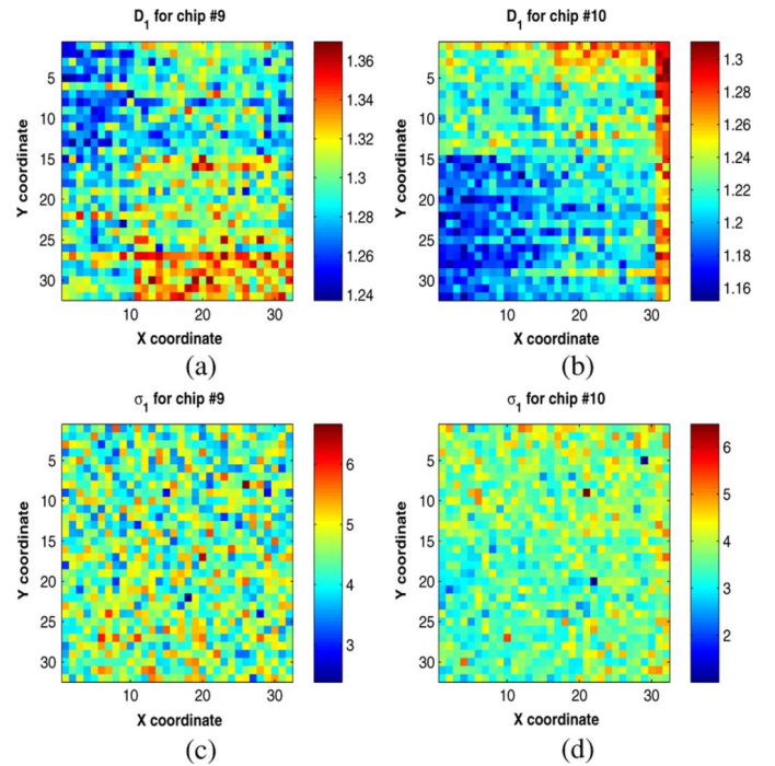
Fig. 11. Extracted parameters d_1 (a), (b) and \sigma_1 (c), (d) for chips 9 and 10.
